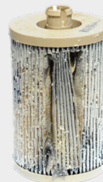
Figure 29 Use of biodiesel of inadequate quality in fuel blends can have negative operational implications
