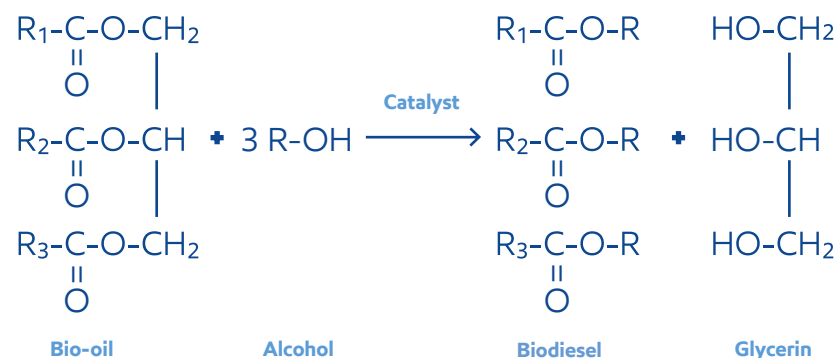
Figure 28 Transesterification process producing biodiesel from bio-oils. For FAME, R is the methyl group (CH 3 )
