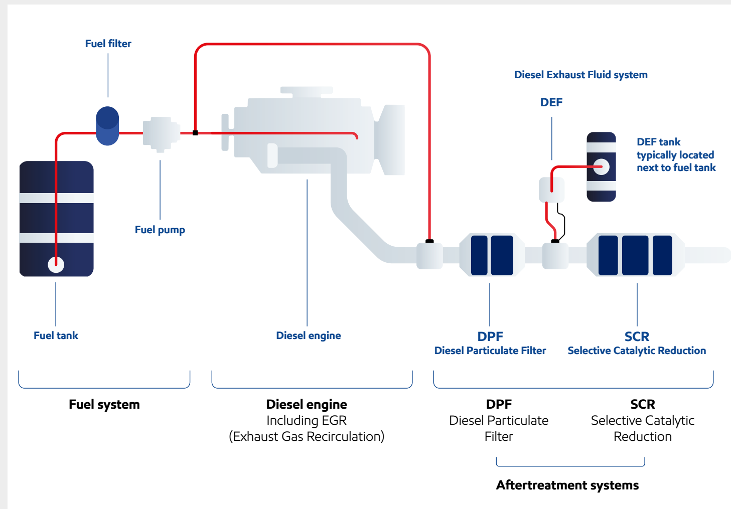
Figure 11 Key elements of a modern lower emission diesel engine
