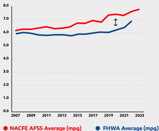
Figure 8 Fleet efficiency improvements in NA 2007-2023 10
